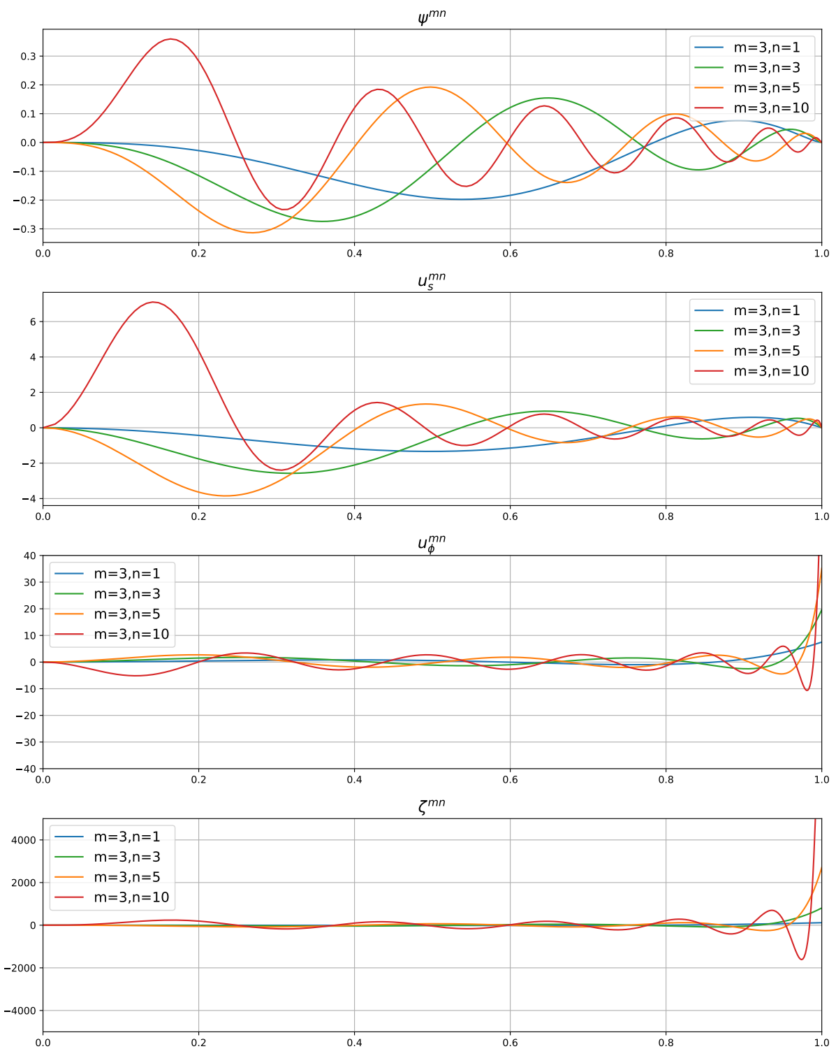
Figure 1.1: The radial bases for streamfunction, equatorial velocity and axial vorticity.
